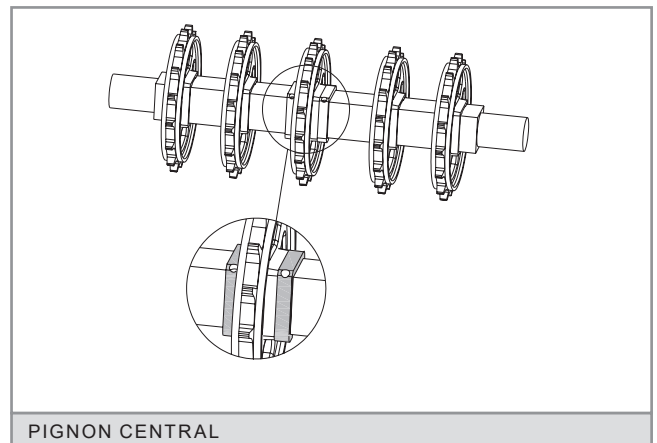
PIGNON CENTRAL
